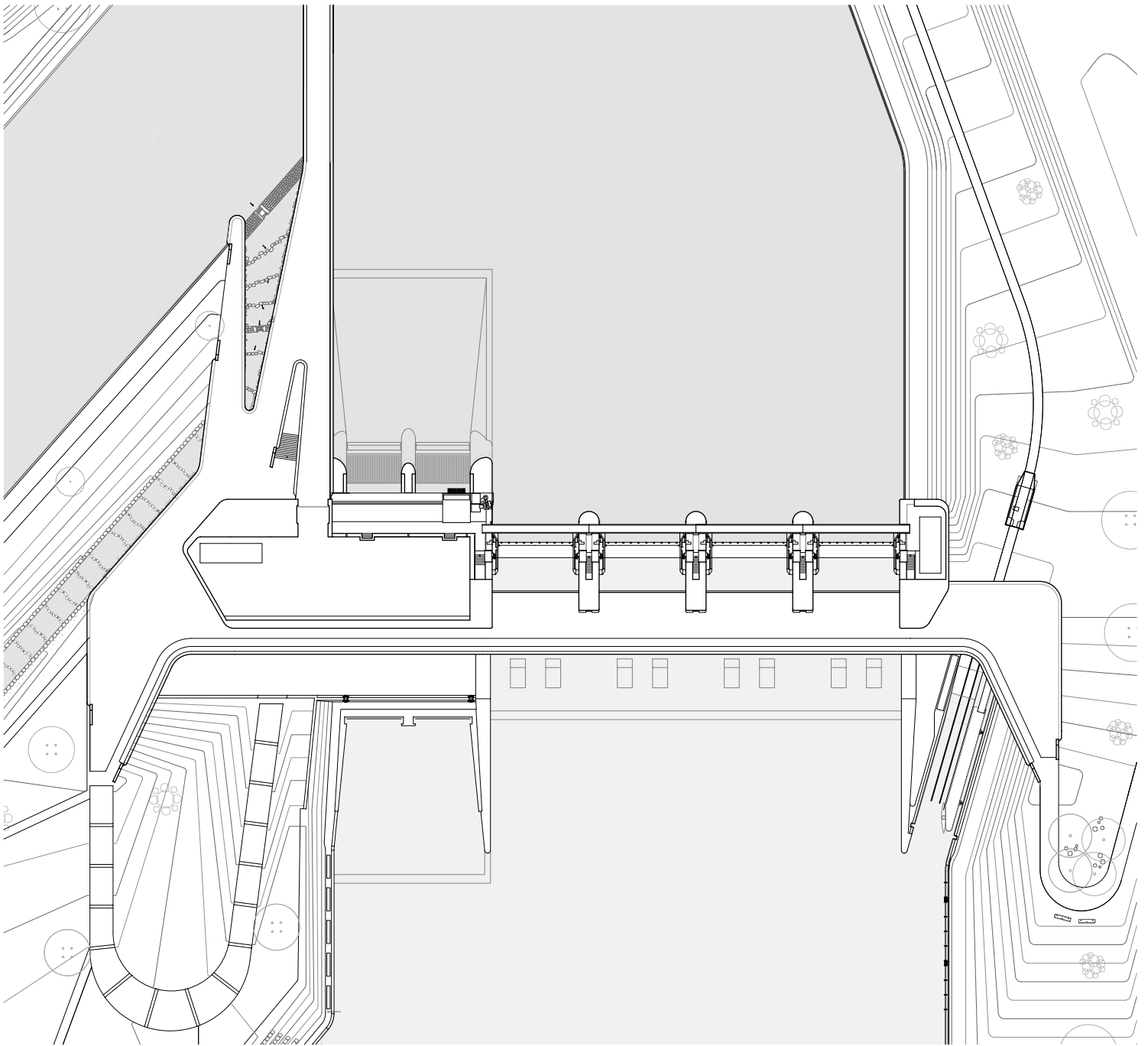
1:500 Grundriss_ +20.00
