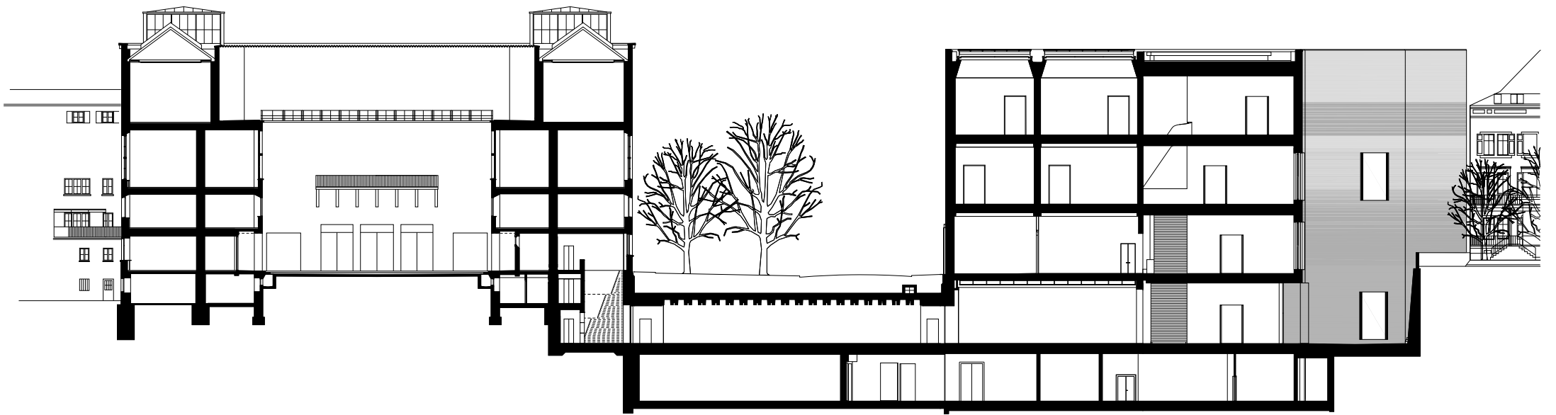
0 1 5 10m Section BB
