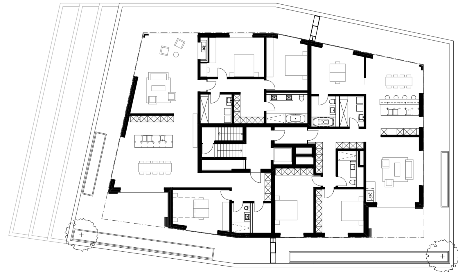
Attika
