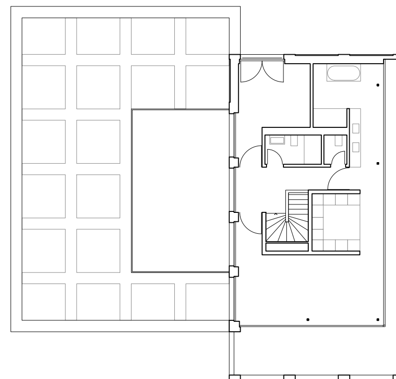
Attikageschoss 1:200
