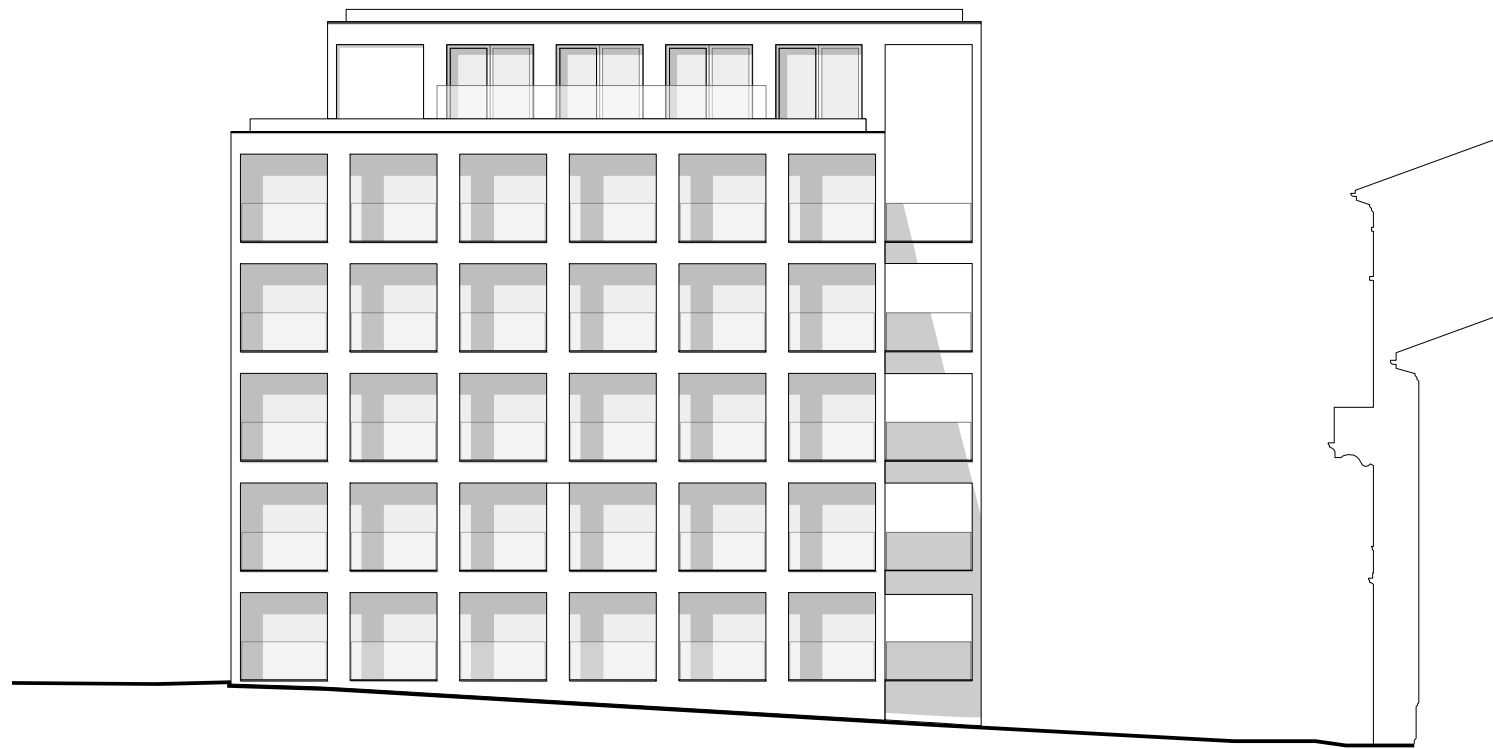
Fassade West 1:200
