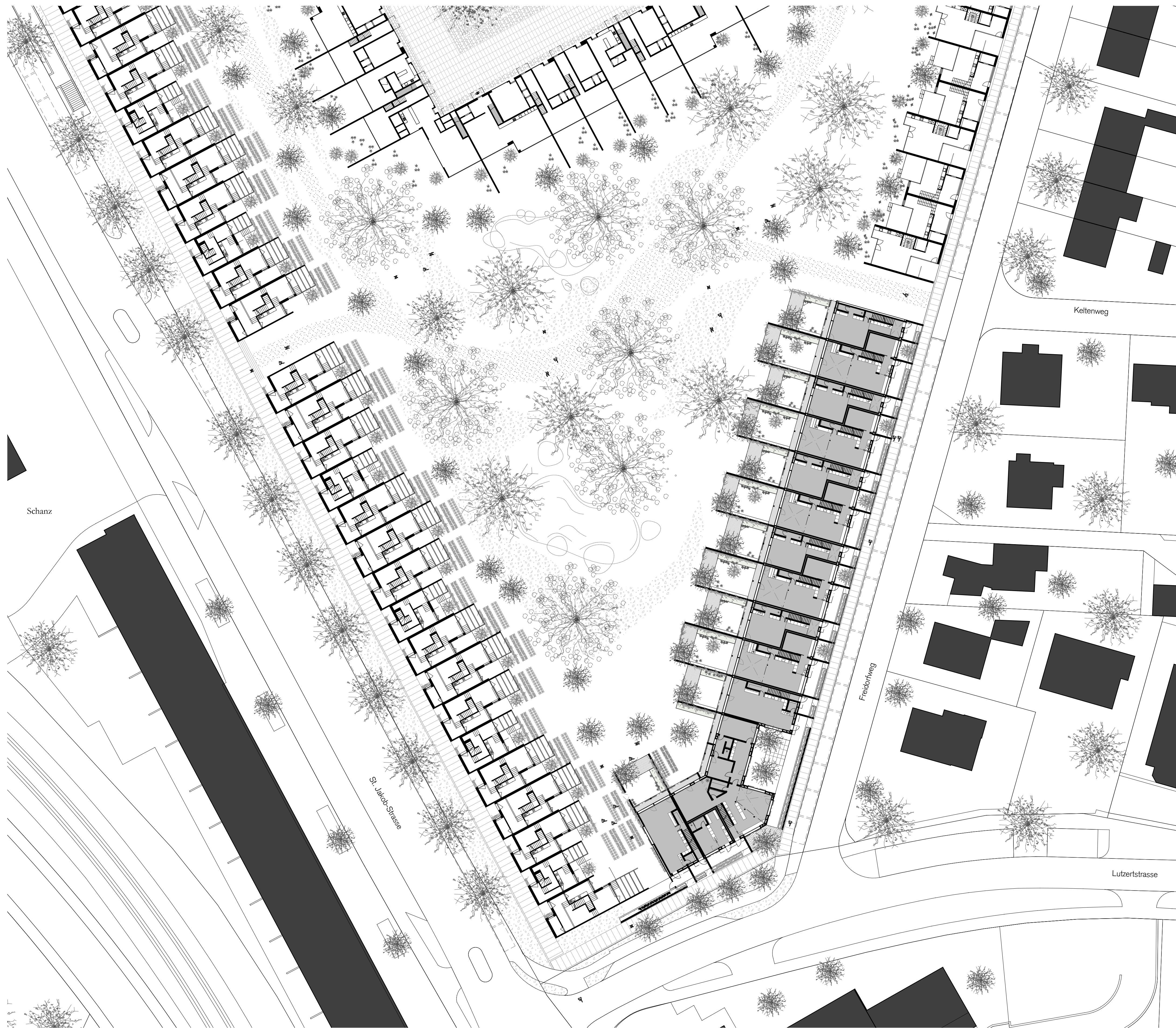
Situationsplan 1:500
